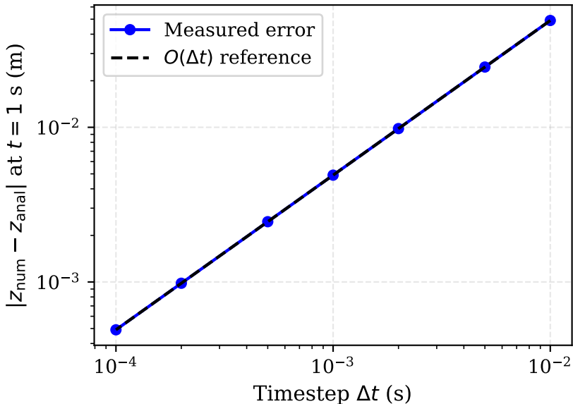
Convergence: error vs timestep
