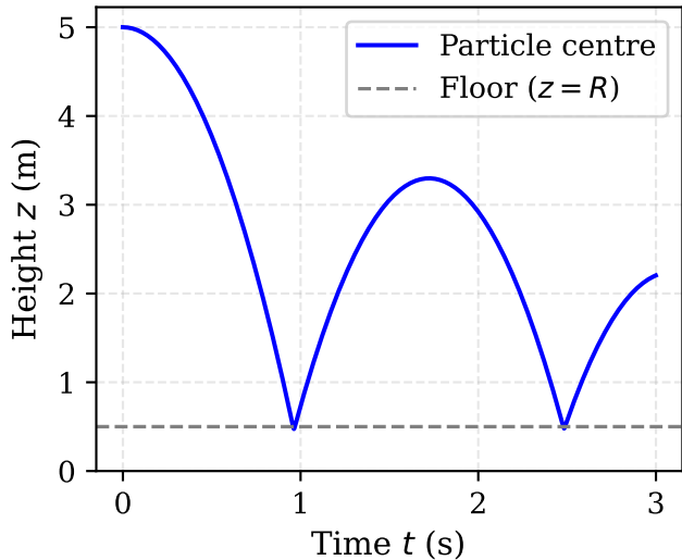
(a) Bounce trajectory
