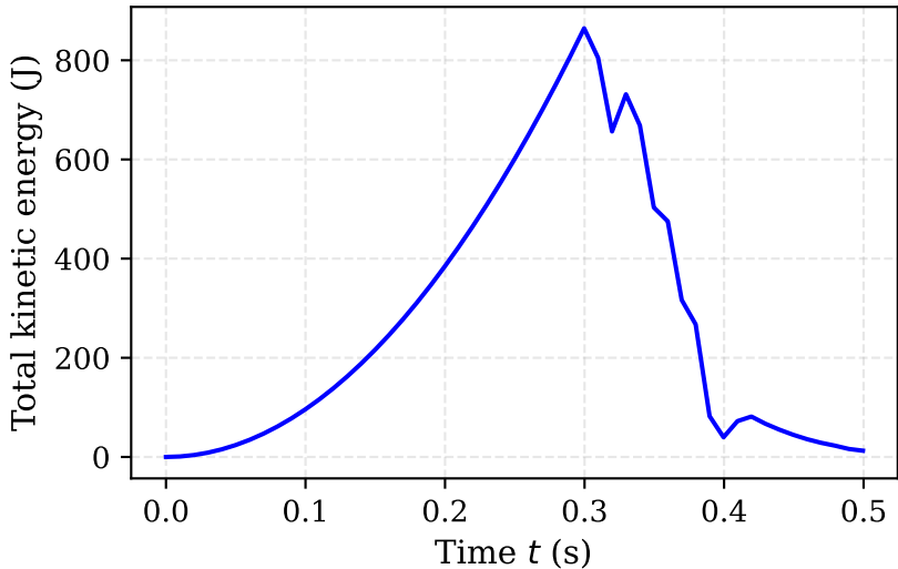
Kinetic energy vs time ( N = 200 )
