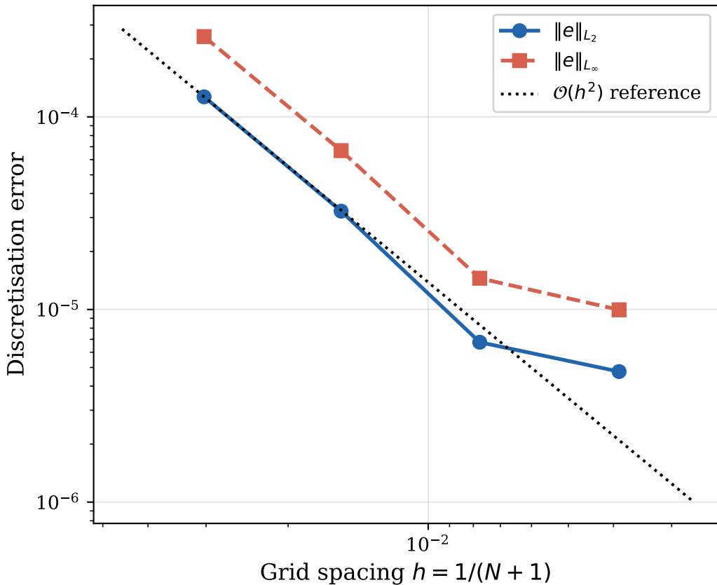
FDM Convergence Study Manufactured solution: T = \sin(\pi x)\sinh(\pi(1 - y))/\sinh(\pi)
