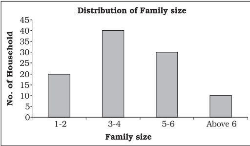
Fig. 8.2: Bar diagram
