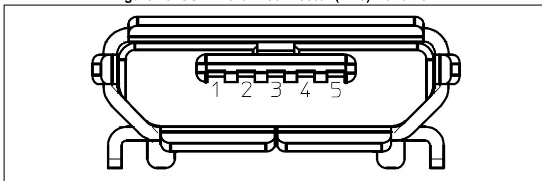
Figure 15. USB Micro-B connector (CN5) front view
