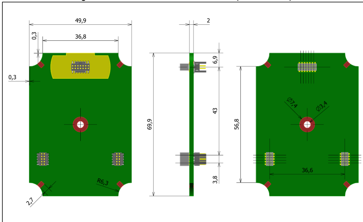
Figure 13. MB1441 mechanical dimensions (in millimeters)
