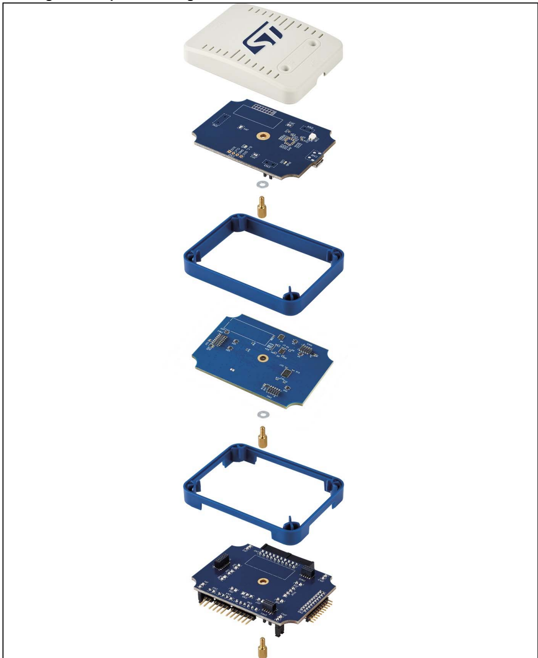
Figure 17. Opened casing for access to all connectors with B-STLINK-VOLT
