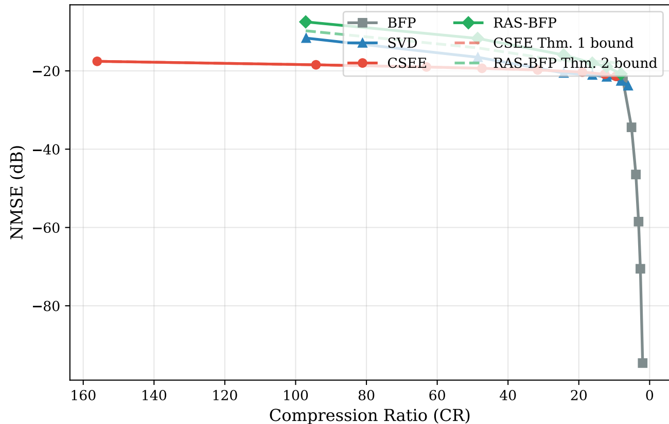
NMSE vs Compression Ratio (M=64, N=1200, SNR=20.0 dB, 3GPP TDL-A)
