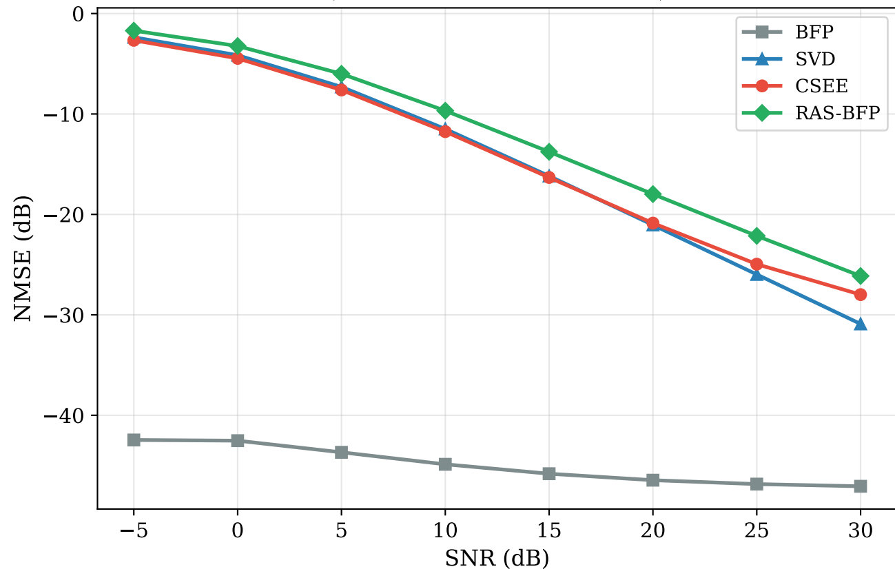
NMSE vs SNR at Fixed Compression (BFP b=8 , r=12/12 , K=300 )
