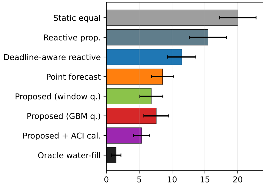
Low-latency cells: violation ratio [%]
