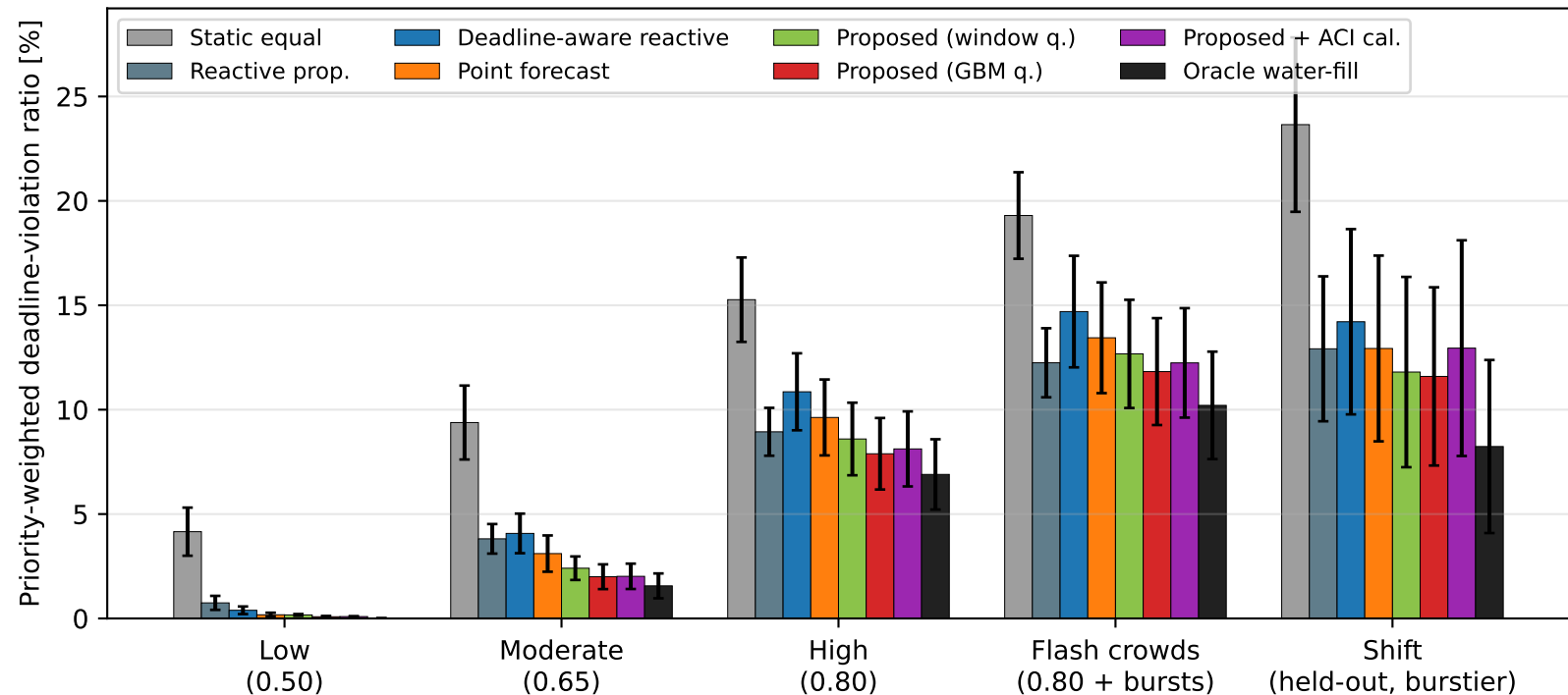
Primary metric per scenario (mean \pm std over 5 test seeds; lower is better)
