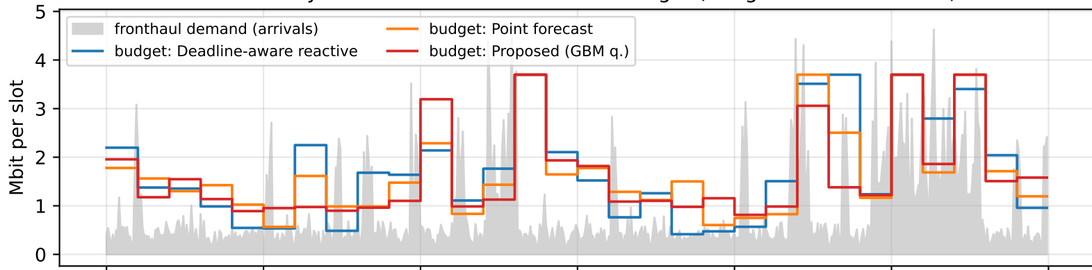
Low-latency cell 0: demand vs. allocated budget (budgets fixed for 10 ms)
