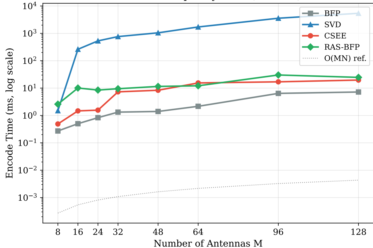
Encoder Complexity vs M (N=1200)
