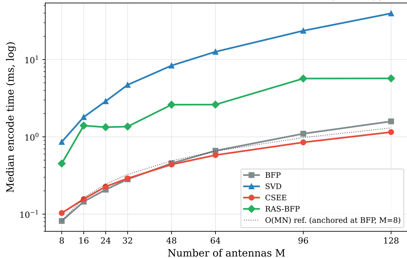
Encoder runtime vs M (N=1200, r=12, K=120, 7 reps, numpy)
