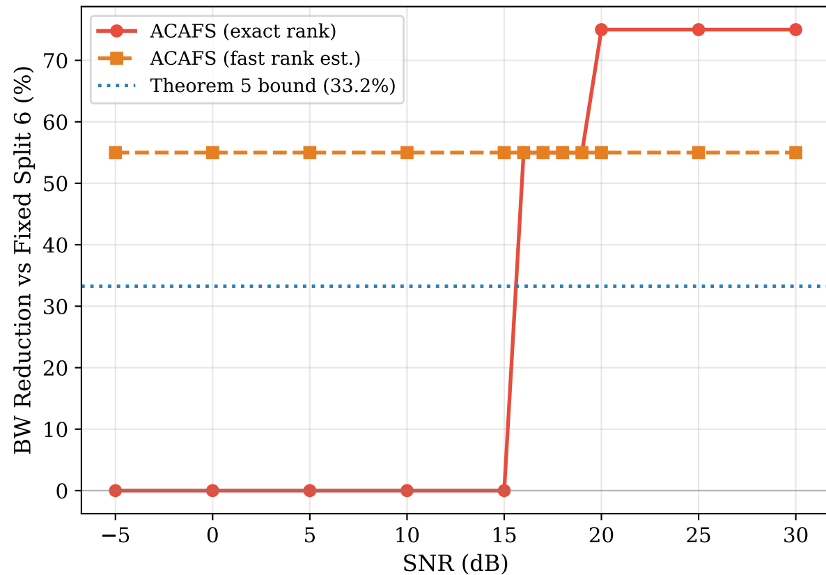
ACAFS Fronthaul Load Reduction
