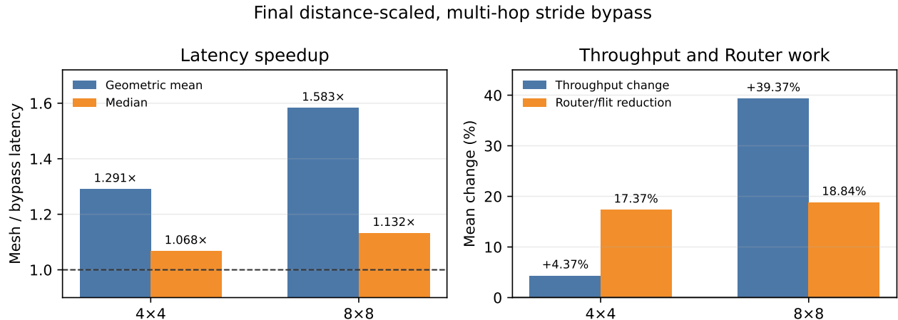
Figure 6: Final bypass results separated by Mesh size. Latency bars report paired-ratio geometric means and medians; throughput and Router-traversal bars report arithmetic mean changes over 768 matched pairs per topology.
