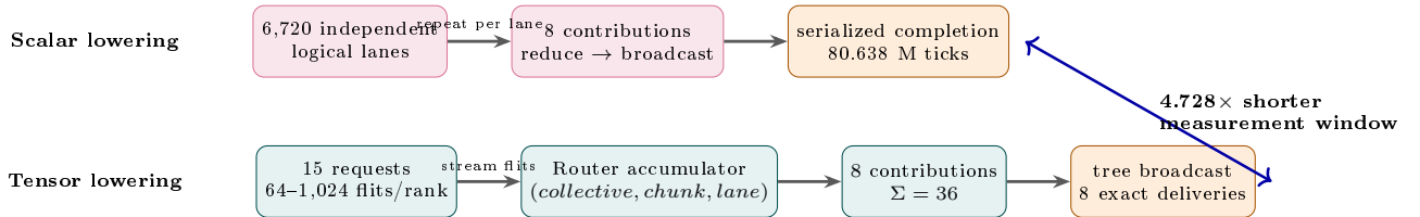
Figure 2: Scalar-lane replay versus the implemented tensor all-reduce path. Tensor mode maintains request/chunk/lane identity while Routers merge eight rank contributions, verify the sum, and multicast the result.
