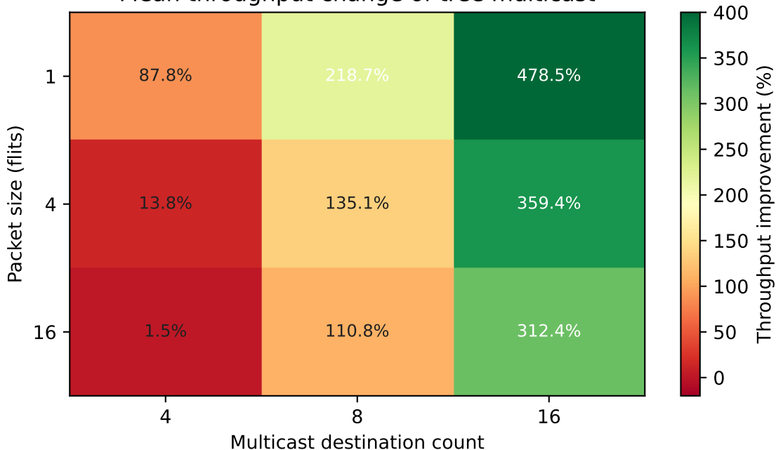
Mean throughput change of tree multicast
