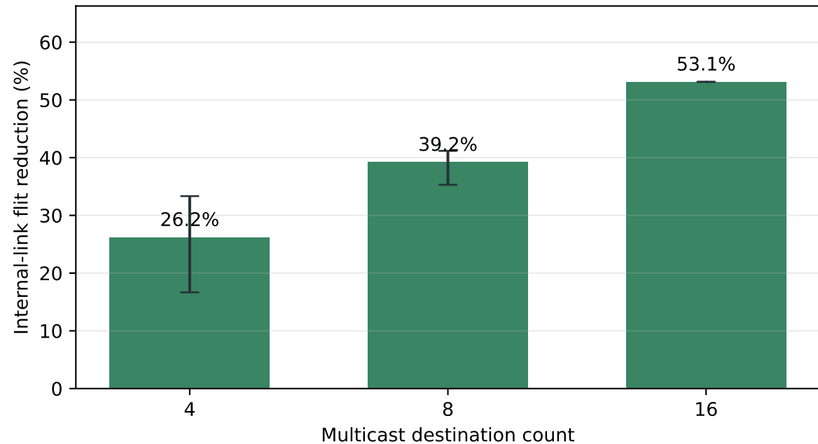
Tree multicast reduces physical link traffic
