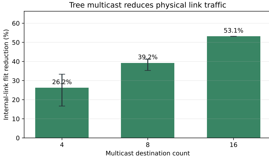
Figure 5: Current-revision multicast internal-link flit reduction. Error bars span observed minima and maxima, not confidence intervals.
