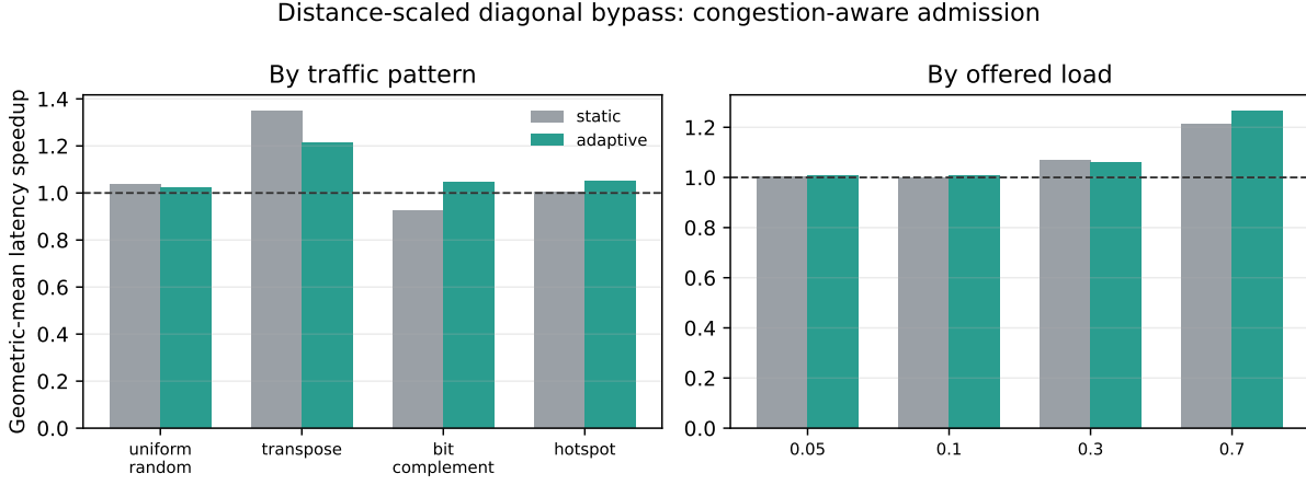
Figure 10: Congestion-aware admission improves the selected physical-wire design across traffic patterns and offered loads while eliminating all regressions larger than 5%.
