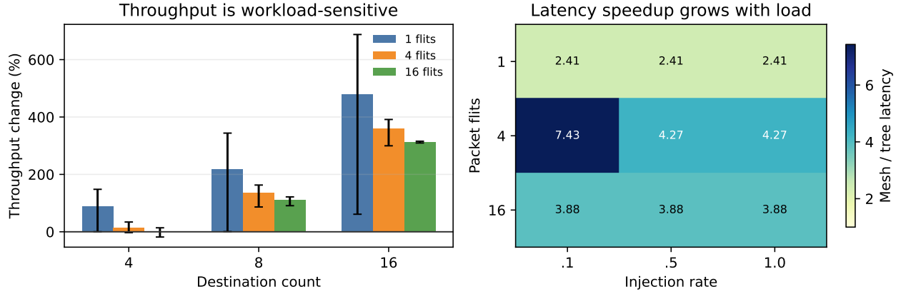
Figure 8: Multicast scaling across destination count, packet size, and load. Bars show mean throughput change with min-max whiskers; the heatmap shows geometric-mean completion-latency speedup across background conditions.
