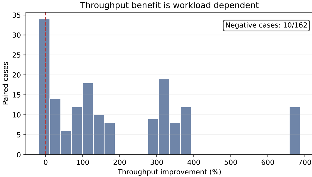
Figure 6: Distribution of multicast throughput change over all 162 paired cases. The dashed line marks unchanged throughput; the ten regressions are all four-destination cases.
