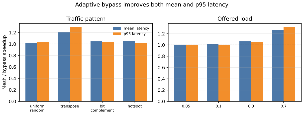
Figure 12: Adaptive bypass latency speedups grouped by traffic pattern and offered load. Bars report geometric means for average latency and p95 latency, exposing both central and tail behavior.
