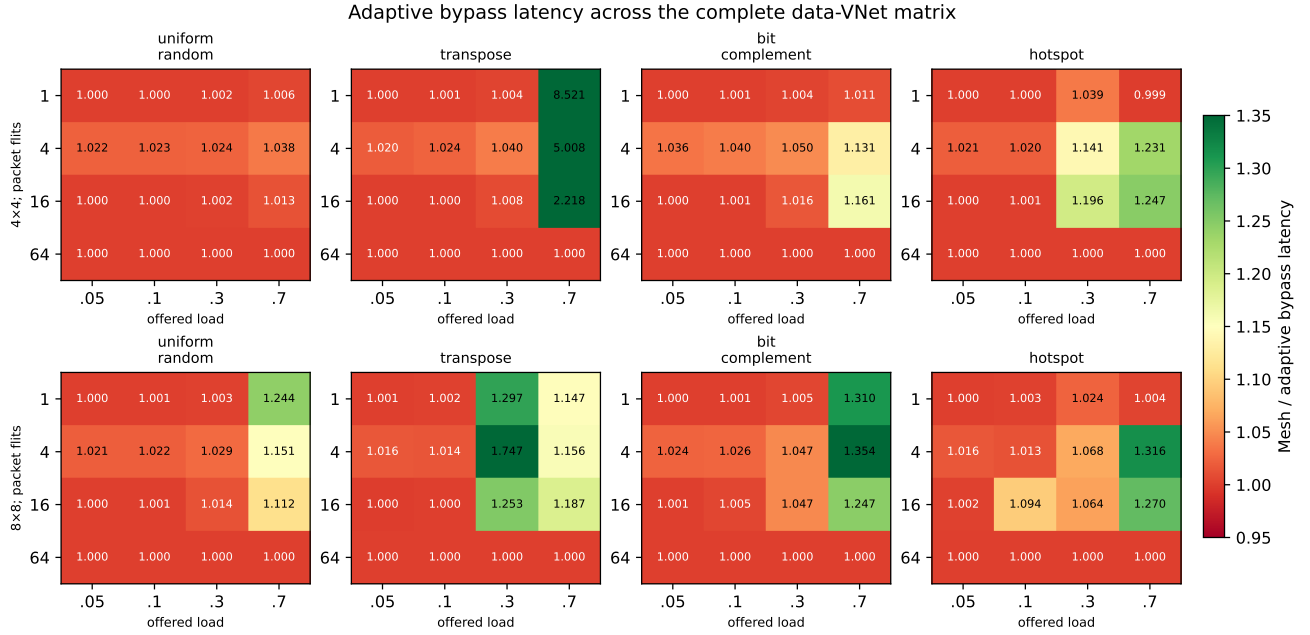
Figure 11: Complete adaptive data-VNet matrix. Each cell is the geometric-mean Mesh/bypass latency speedup over three seeds; rows separate mesh size, columns traffic pattern, and each panel enumerates packet length (rows) and offered load (columns). Values above 1 indicate a bypass benefit.
