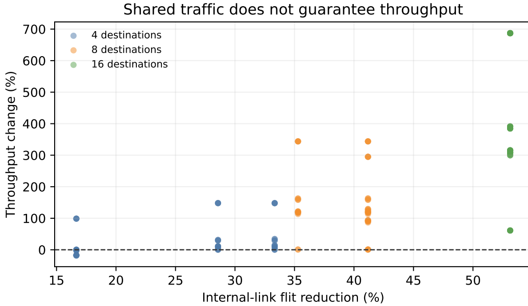
Figure 9: Paired multicast cases: internal-link flit reduction versus throughput change. Color denotes destination count; the dashed line marks unchanged throughput.
