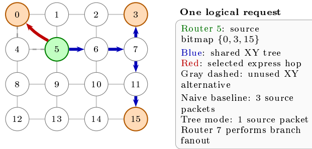
Figure 3: Integrated multicast and bypass example on a 4 \times 4 Mesh. Cost-aware routing uses an express hop for an isolated destination but keeps the shared XY prefix for the other destinations. The diagram shows logical structure; link timing is evaluated separately by the two wire models.
