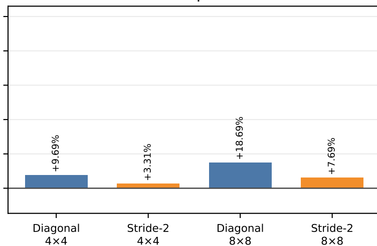
Transpose
