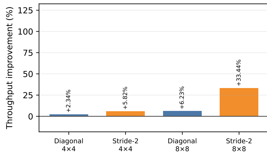
Uniform random
