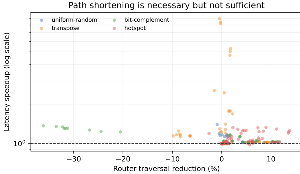
Figure 10: Mechanism-level trade-off for adaptive bypass. Each point is one traffic/size/load/flit aggregate; the x-axis is Router-traversal reduction and the y-axis is Mesh-relative latency speedup. Color identifies traffic.
