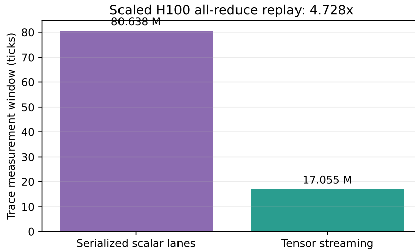
Figure 11: Same scaled H100 all-reduce trace and topology: tensor streaming versus serialized scalar-lane lowering. The p95 values are not compared because their granularity differs.
