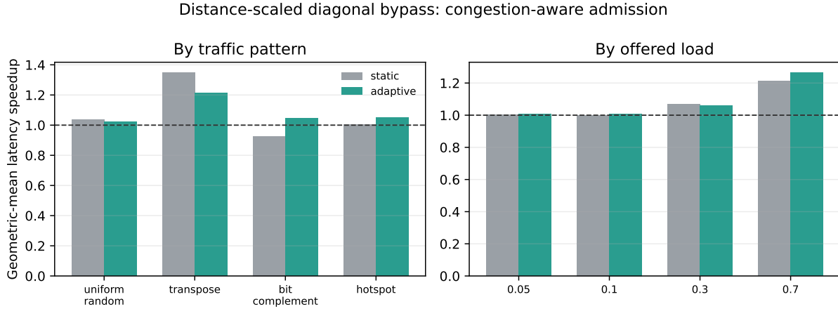
Figure 7: Congestion-aware admission improves the selected physical-wire design across traffic patterns and offered loads while eliminating all regressions larger than 5%.
