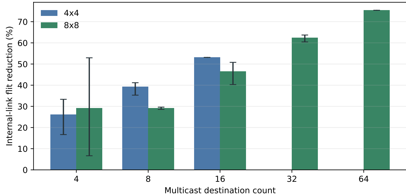
Tree multicast traffic reduction across Mesh sizes
