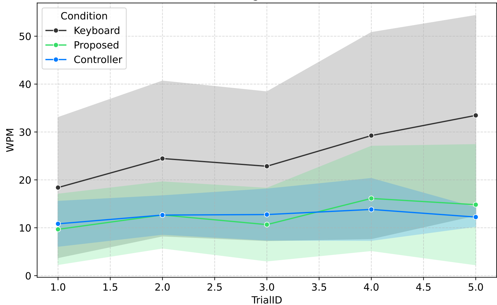
WPM Learning Curve (Practice)
