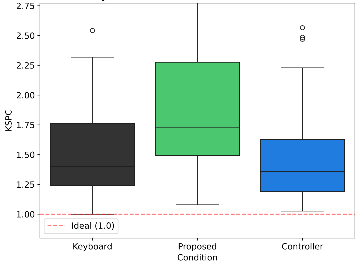
Keystrokes Per Character (KSPC) (Practice)
