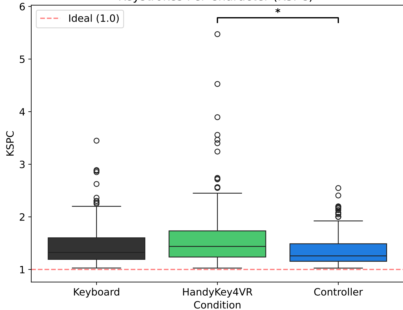
Keystrokes Per Character (KSPC)
