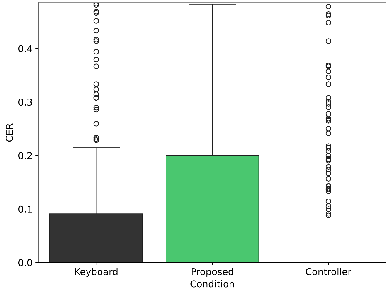
Character Error Rate (CER)
