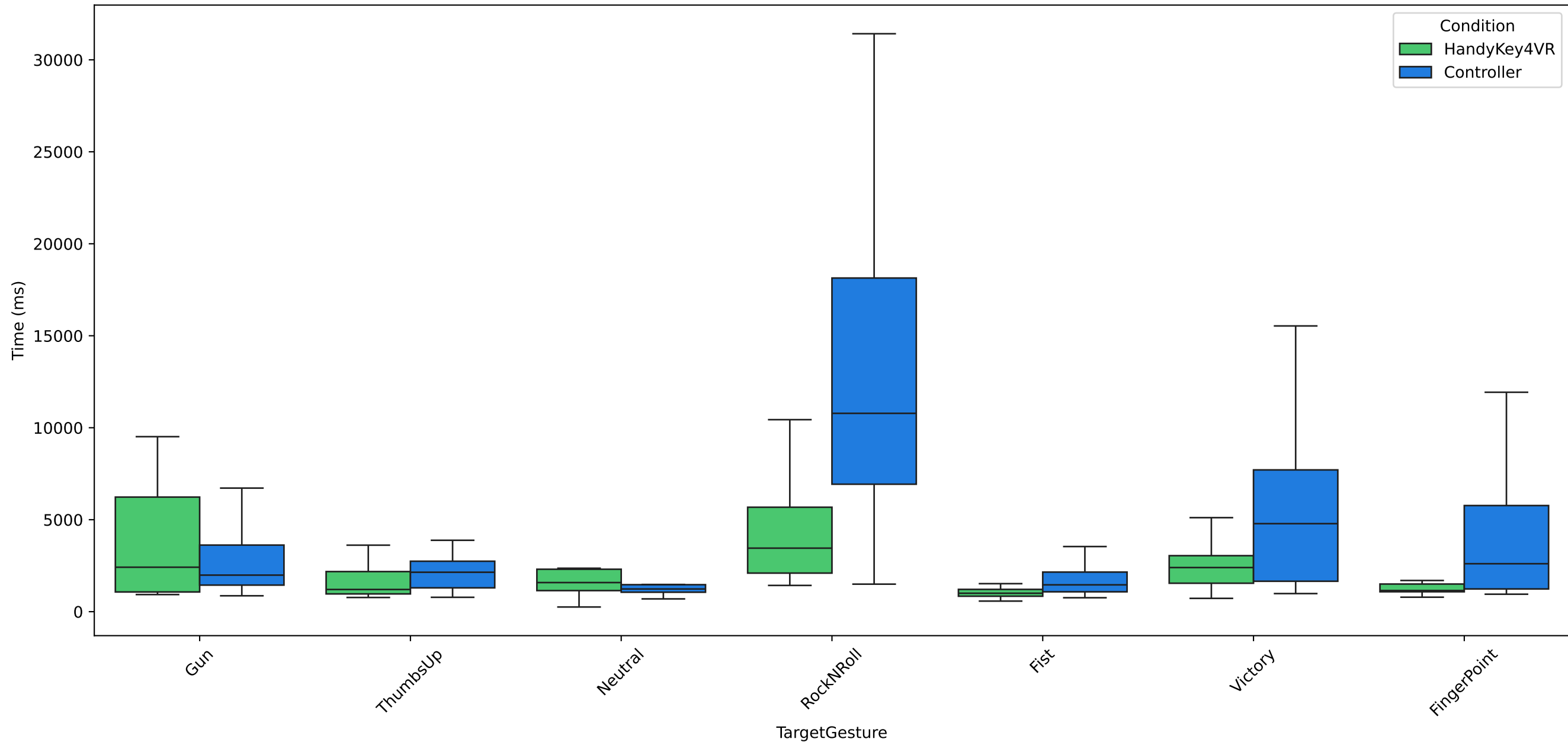
Reaction Time by Gesture Type (Practice)
