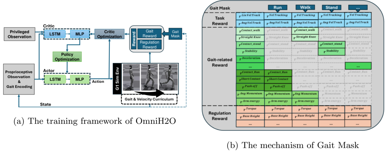
Fig. 1.4: Overview of the proposed gait-conditioned reinforcement learning method. (a) illustrates the policy network architecture with gait encoding, and (b) shows the dynamic reward composition using the Gait Mask (source: [4]).
