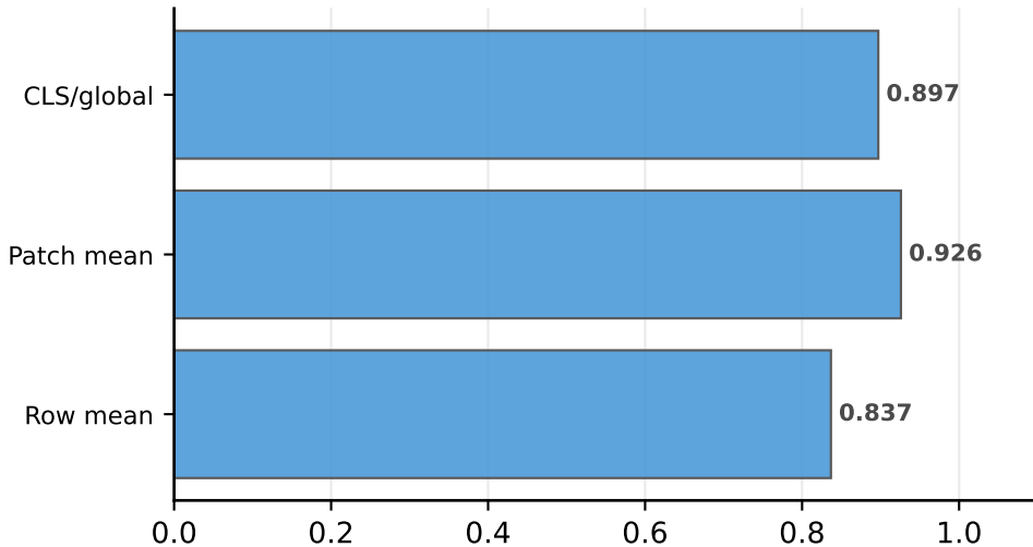
Accuracy
