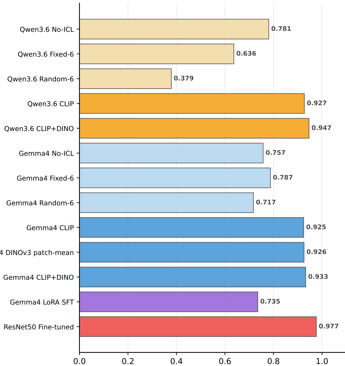
Accuracy
