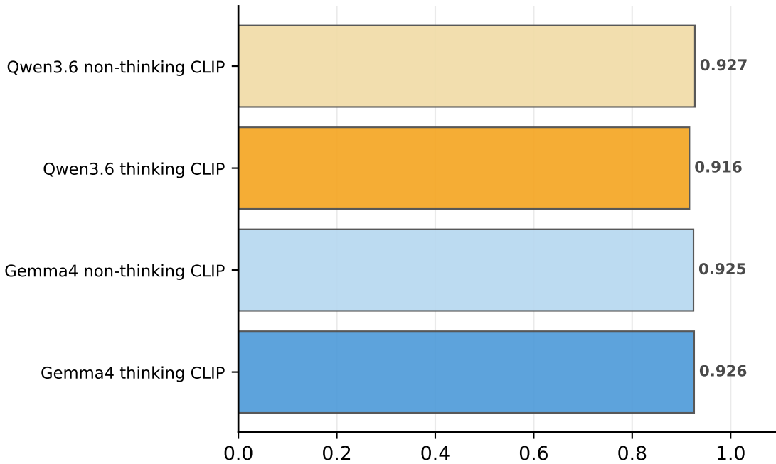
Accuracy
