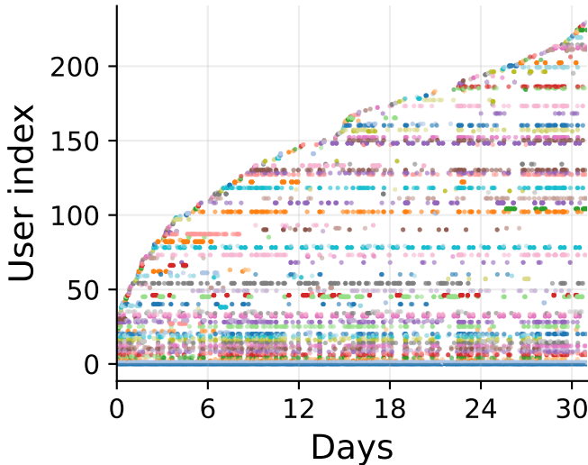
Model rank 41
