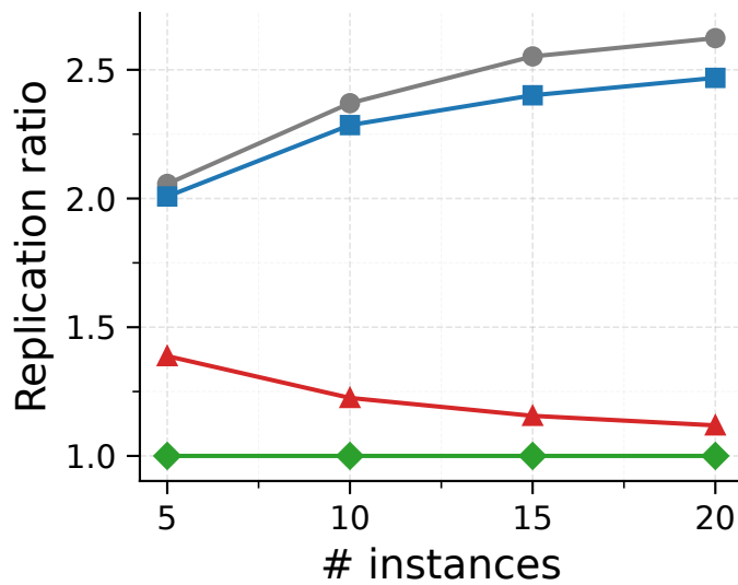
(c) Replication vs instance count
