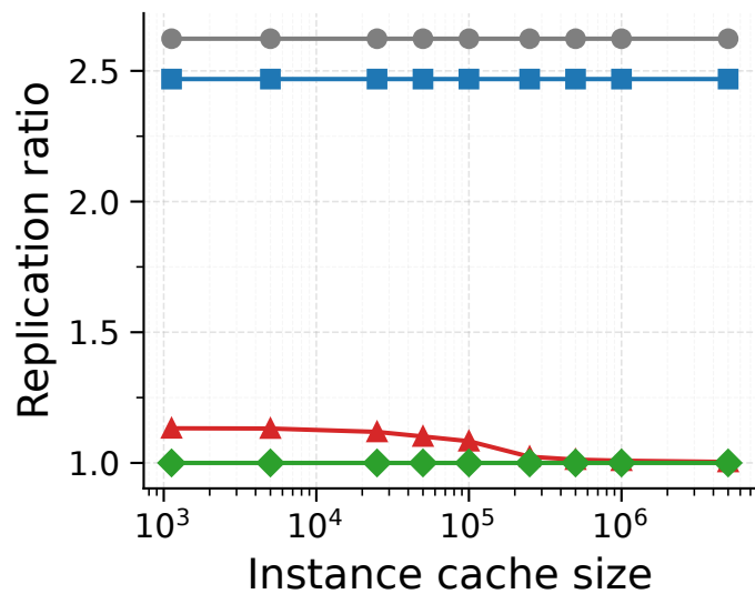
(b) Replication vs cache size
