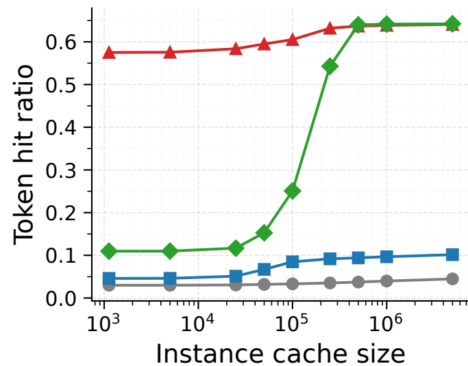
(a) Hit ratio vs cache size
