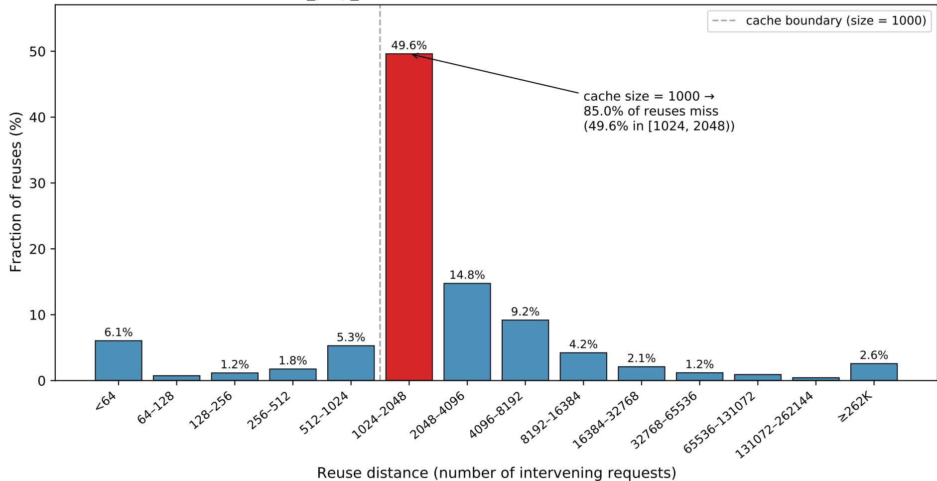
msr_prxy_0: reuse distance distribution (12.4M reuses)
