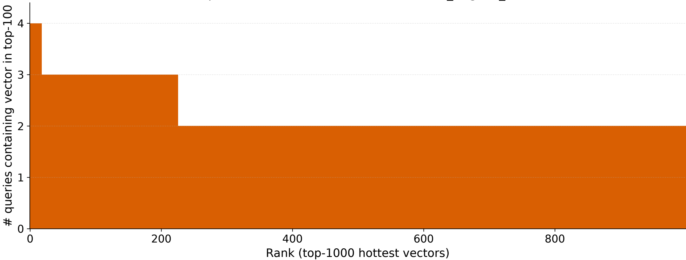
Top-1000 hottest vectors, codesearchnet_original_v0
