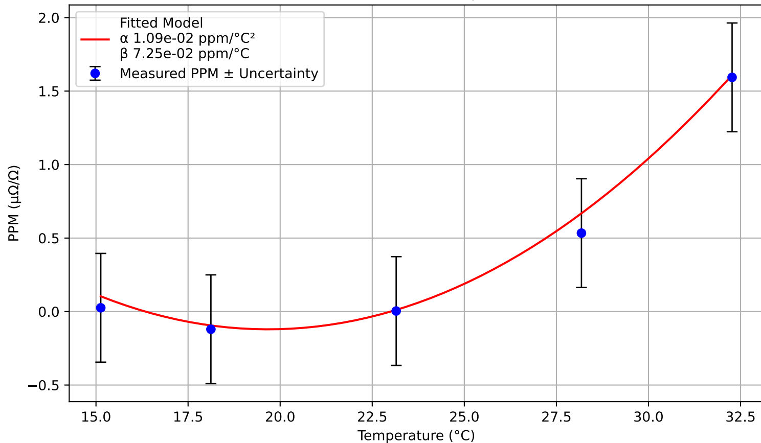
PPM Deviation vs Temperature
