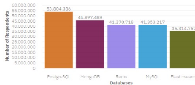
Top 5 Desired Database to Learn
