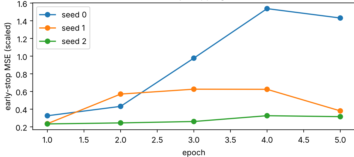
Early stopping
