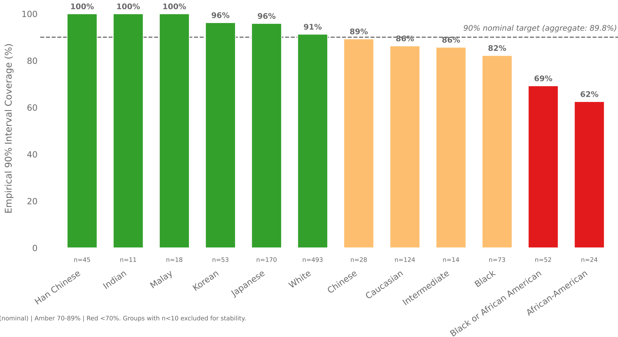
MAPIE Conformal Prediction Coverage by Ancestry Subgroup (IWPC-6256)
