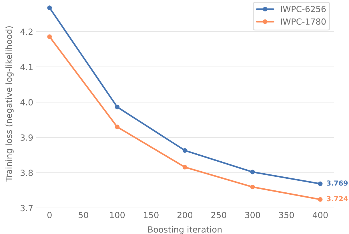
NGBoost Natural-Gradient Training Loss
