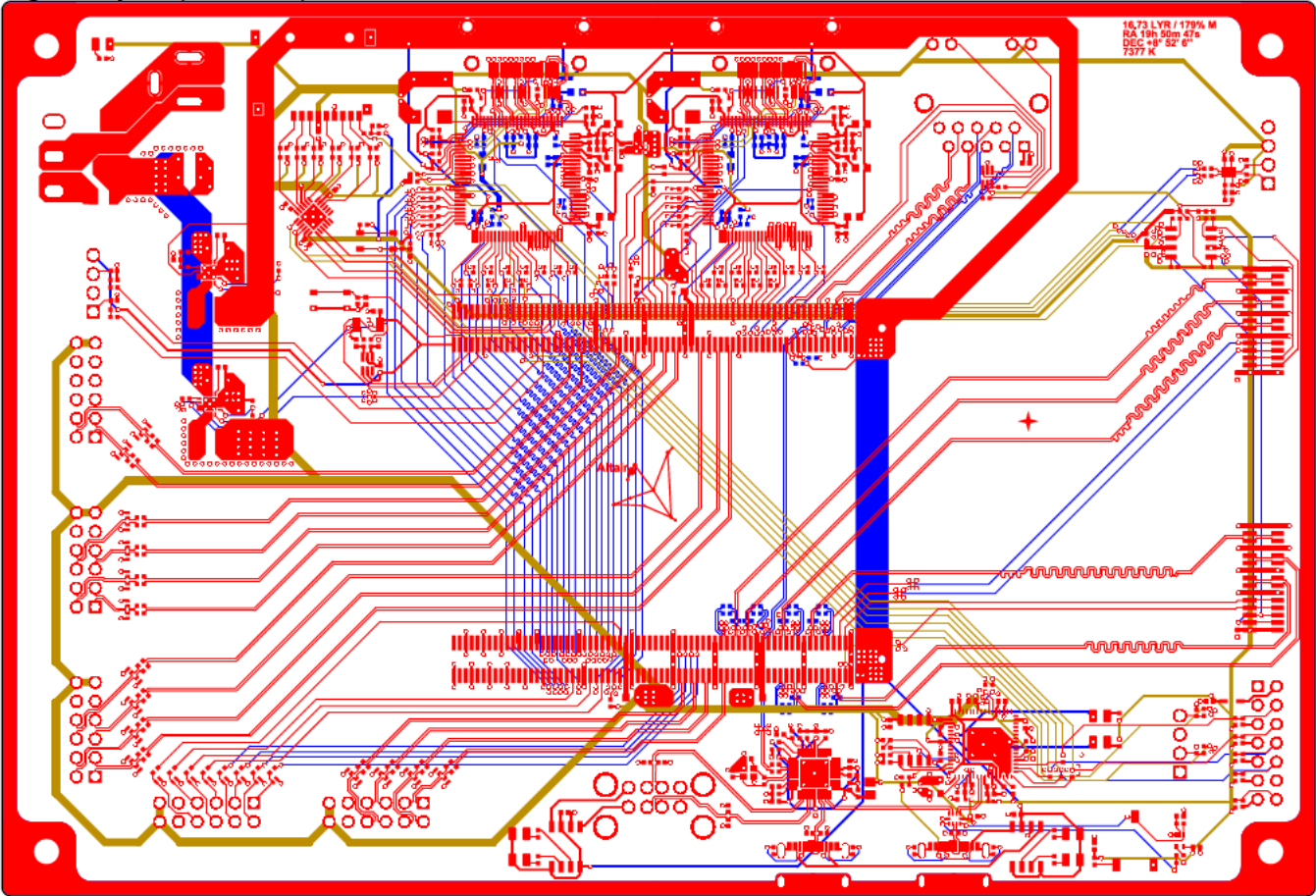
Signal Layers (Scale 1:1)
