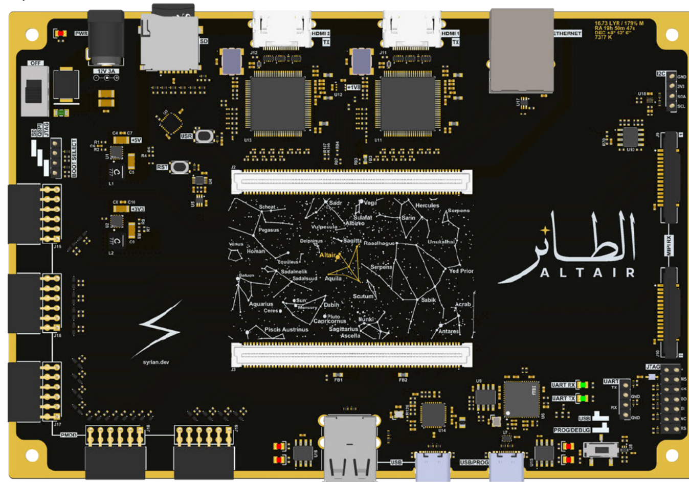
Top 3D View
