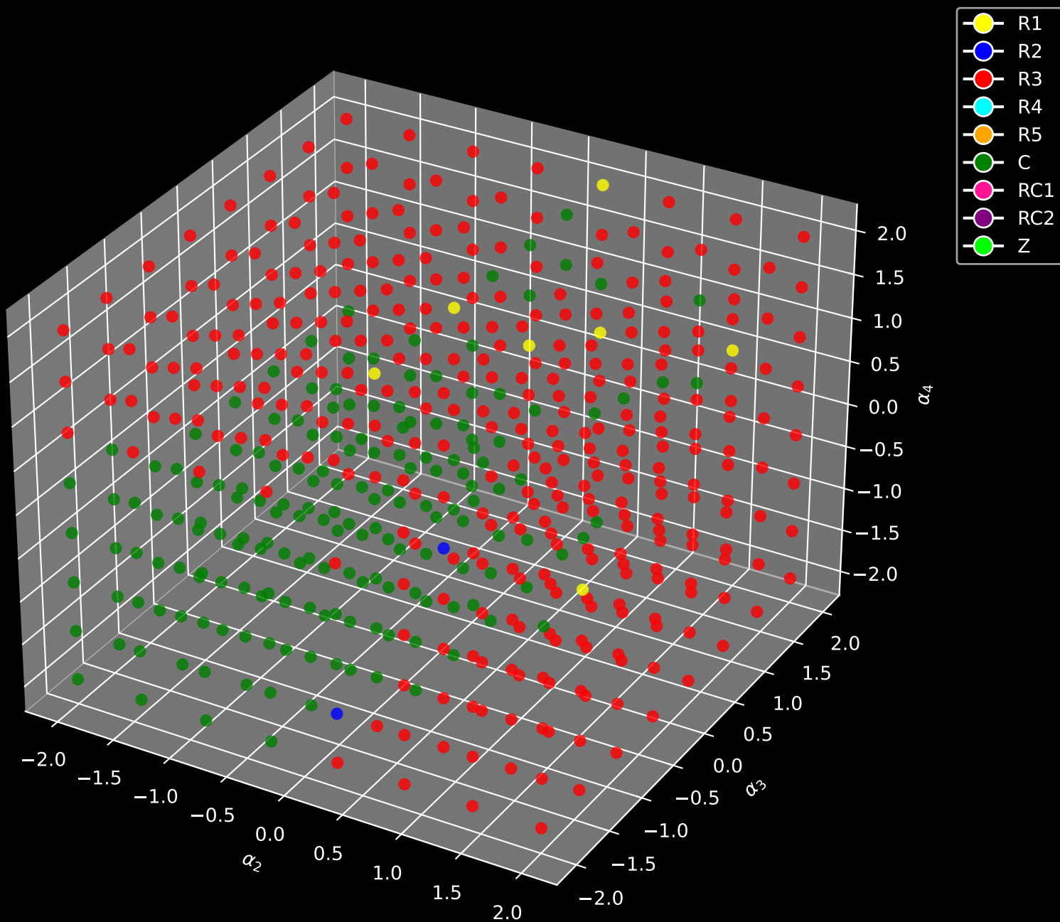
Eigenvalue Categorization (Fixed \alpha_1 = 0.10 )
