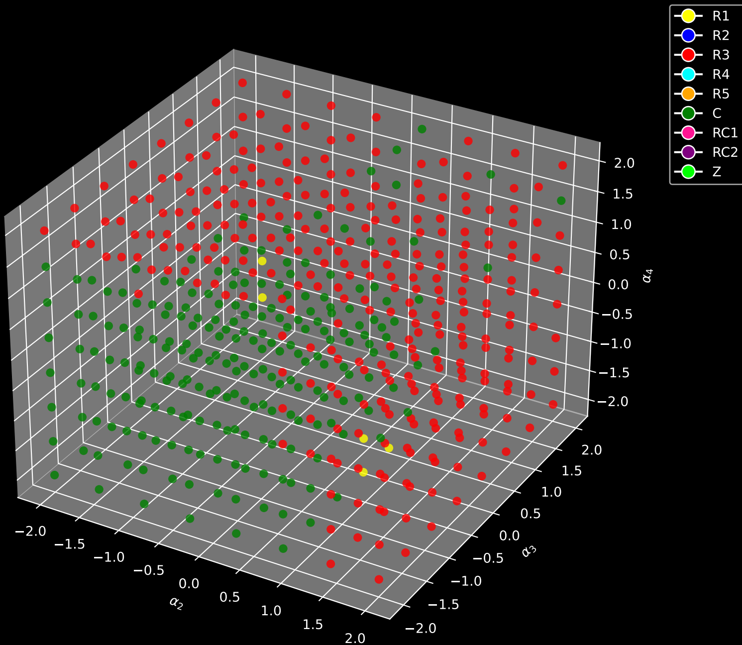
Eigenvalue Categorization (Fixed \alpha_1 = 1.30 )
