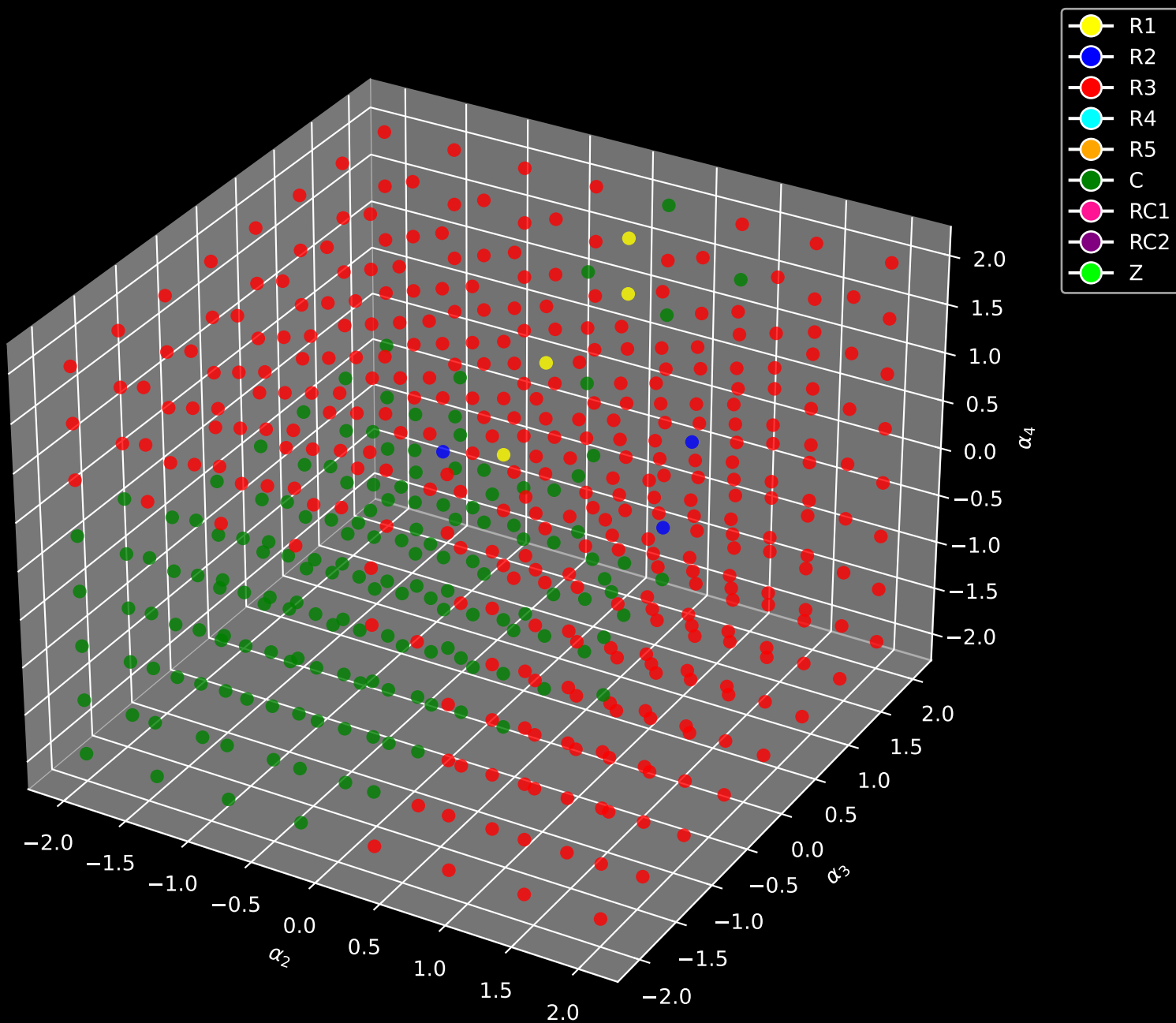
Eigenvalue Categorization (Fixed \alpha_1 = -0.50 )
