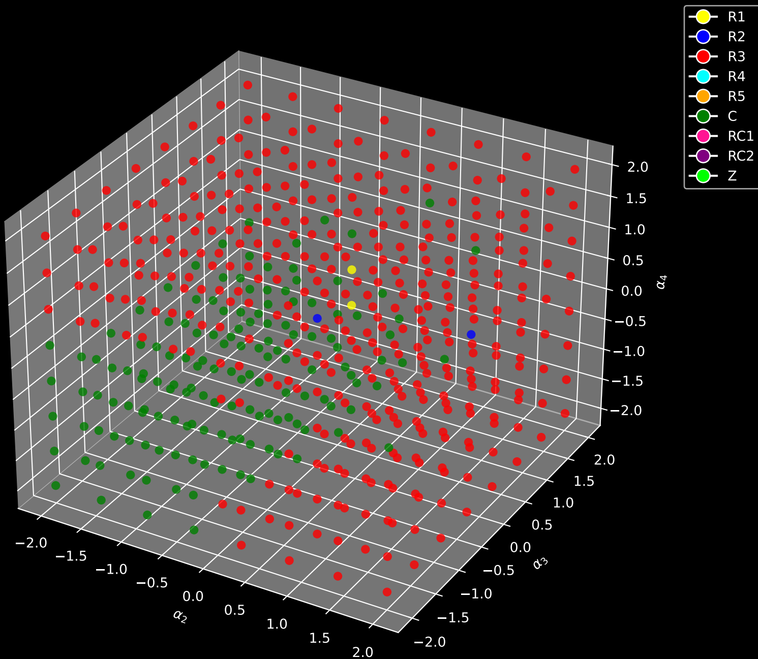
Eigenvalue Categorization (Fixed \alpha_1 = -1.10 )
