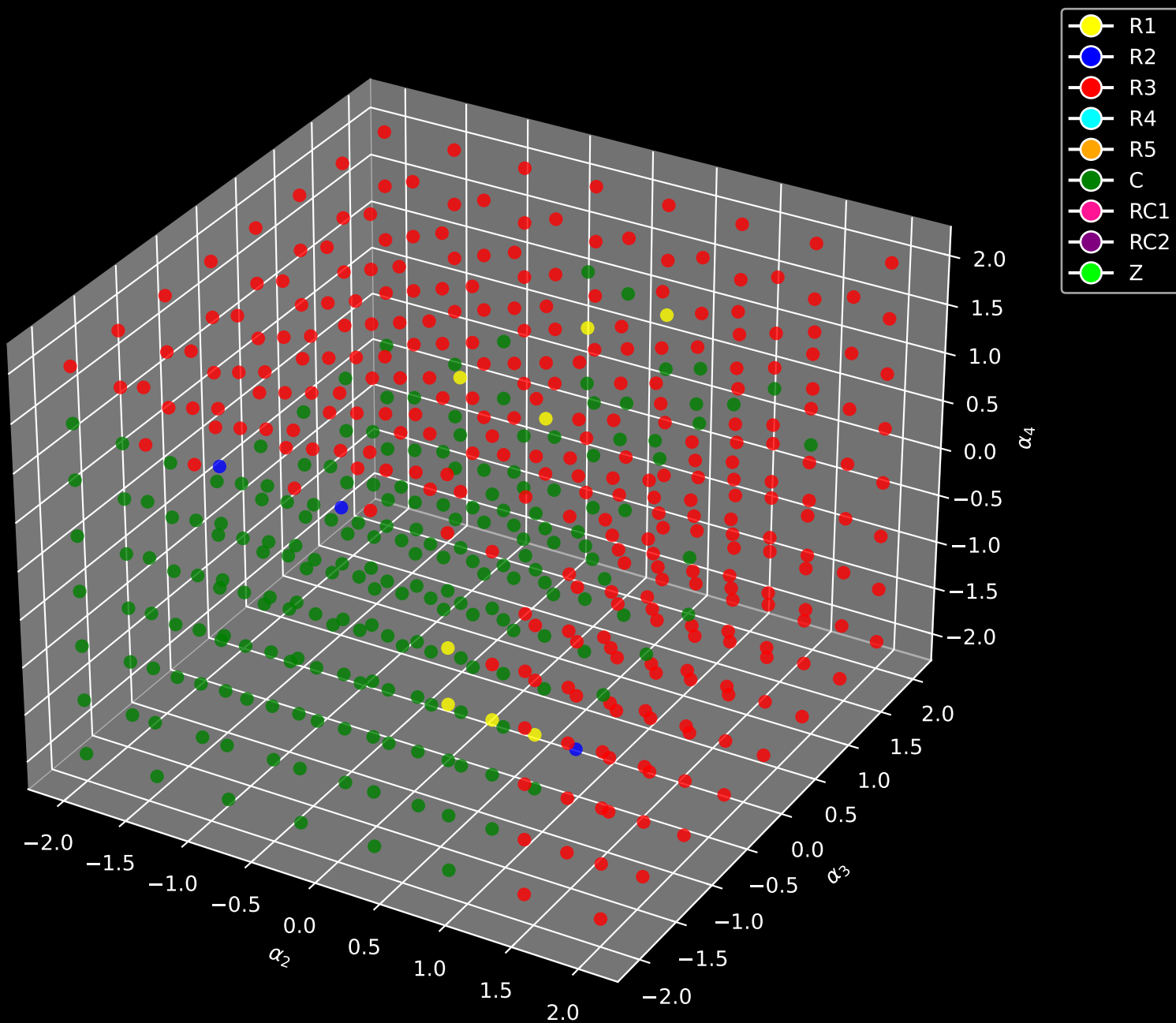
Eigenvalue Categorization (Fixed \alpha_1 = 1.00 )
