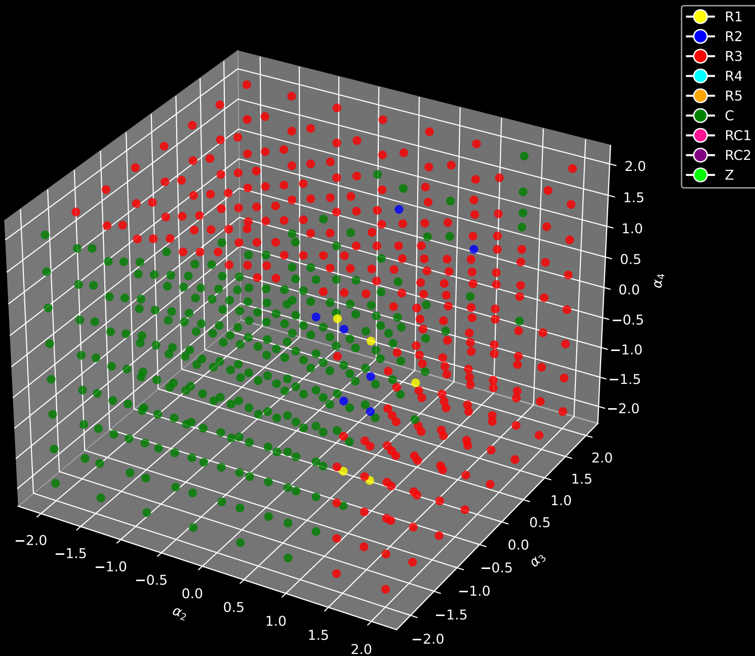
Eigenvalue Categorization (Fixed \alpha_1 = 1.90 )
