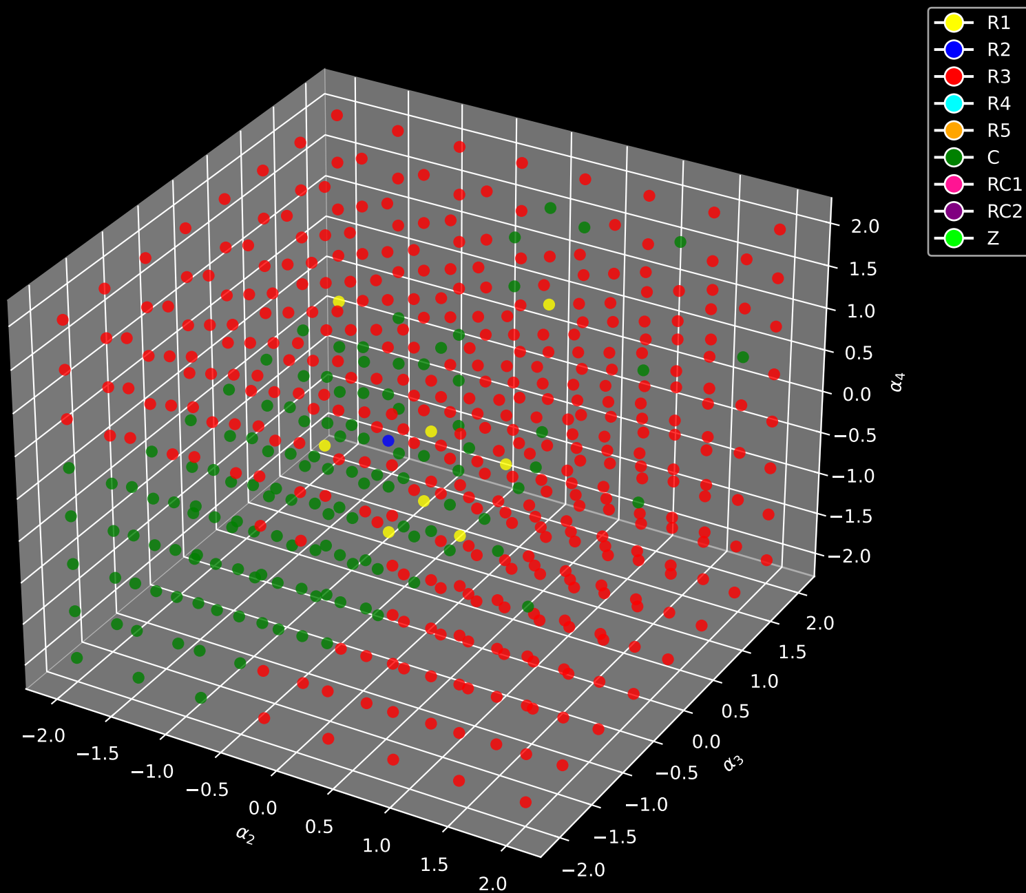
Eigenvalue Categorization (Fixed \alpha_1 = -1.70 )
