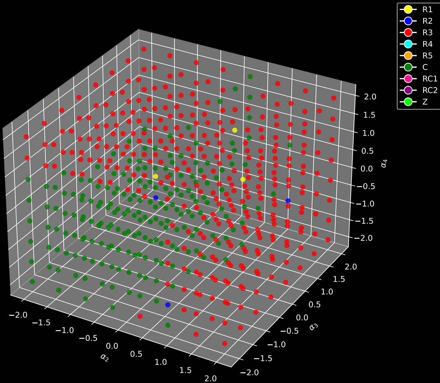
Eigenvalue Categorization (Fixed \alpha_1 = 0.40 )
