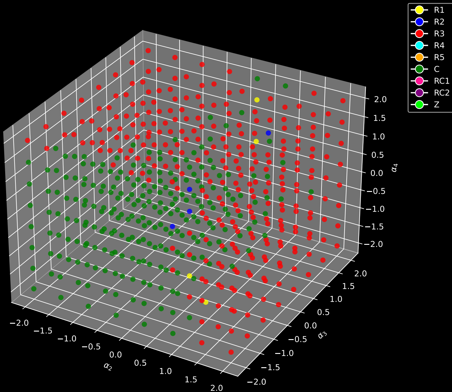
Eigenvalue Categorization (Fixed \alpha_1 = 1.60 )
