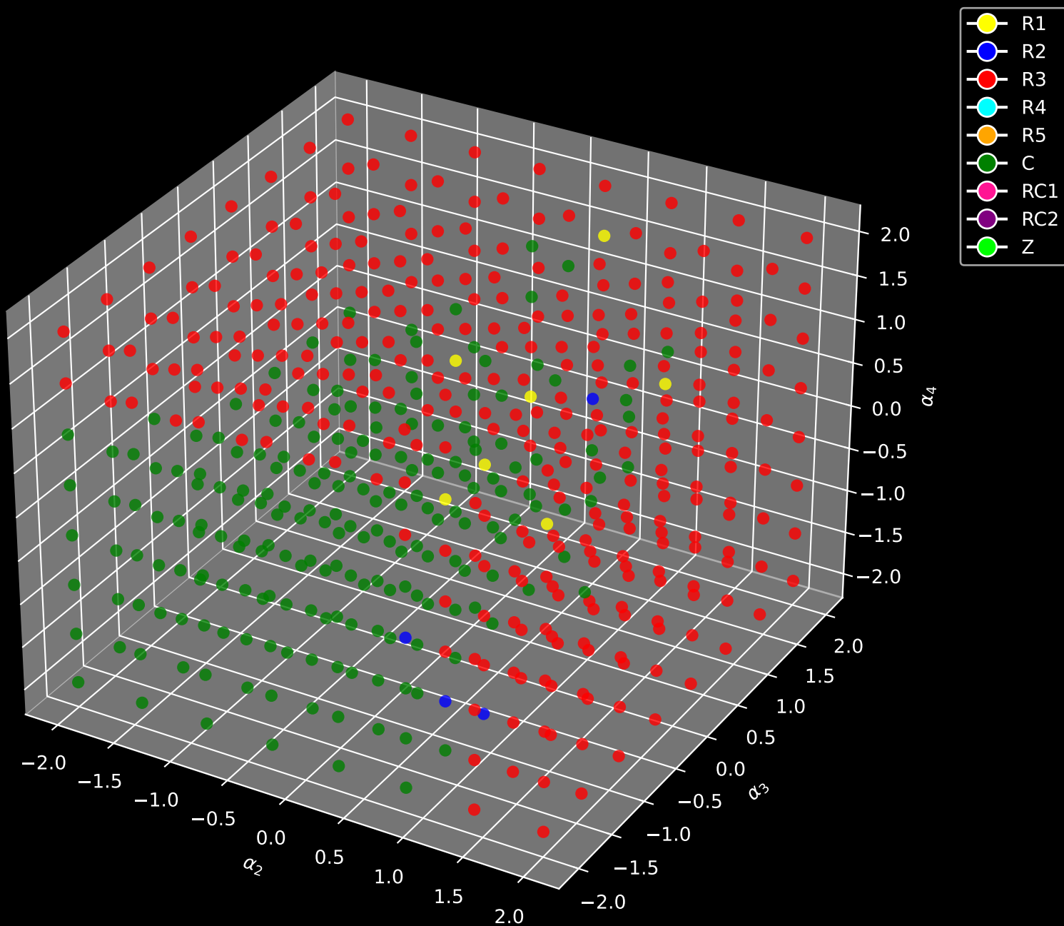
Eigenvalue Categorization (Fixed \alpha_1 = 0.70 )
