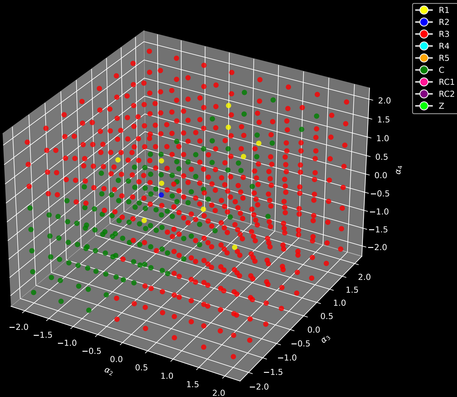
Eigenvalue Categorization (Fixed \alpha_1 = -2.00 )
