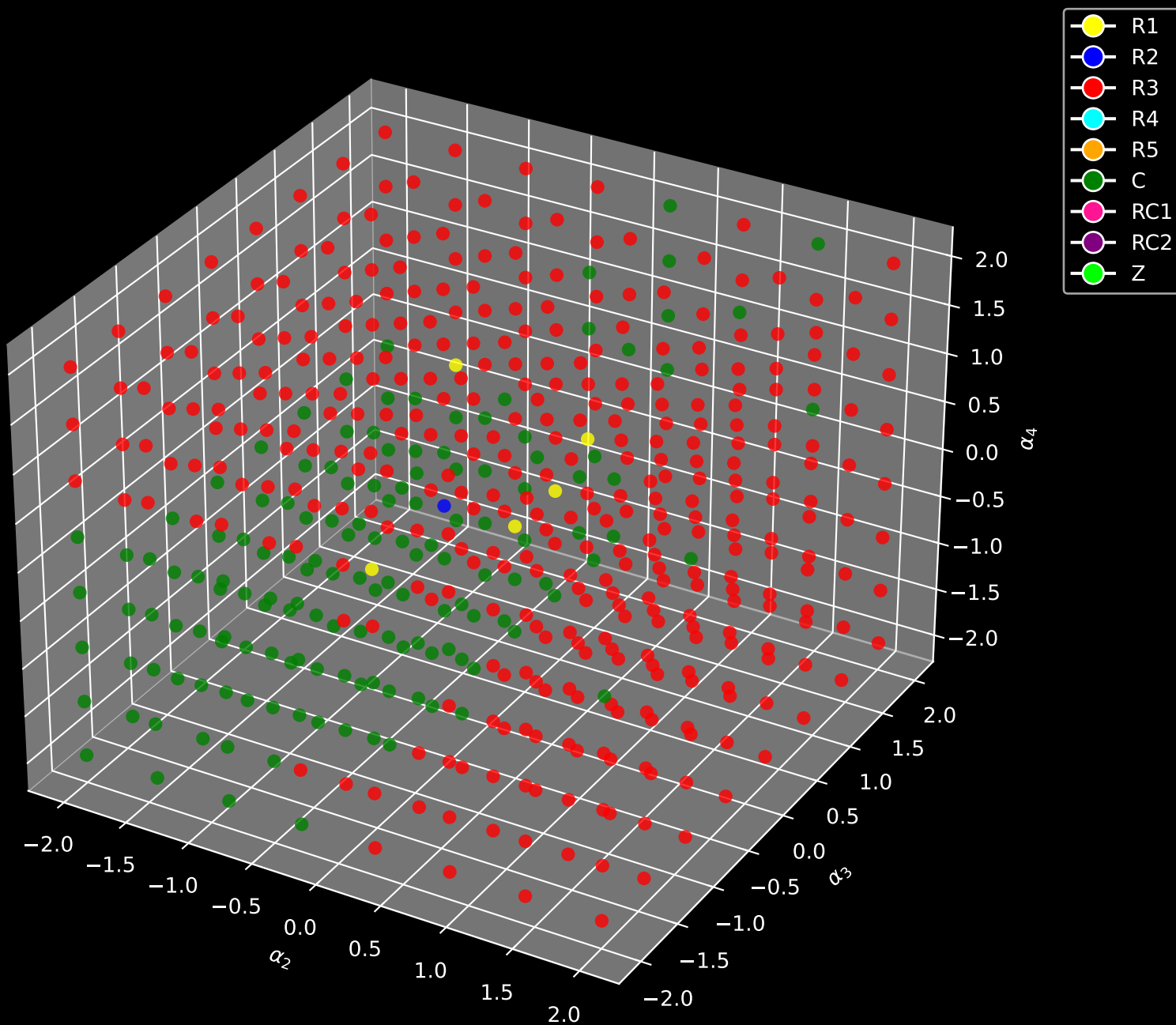
Eigenvalue Categorization (Fixed \alpha_1 = -1.40 )
