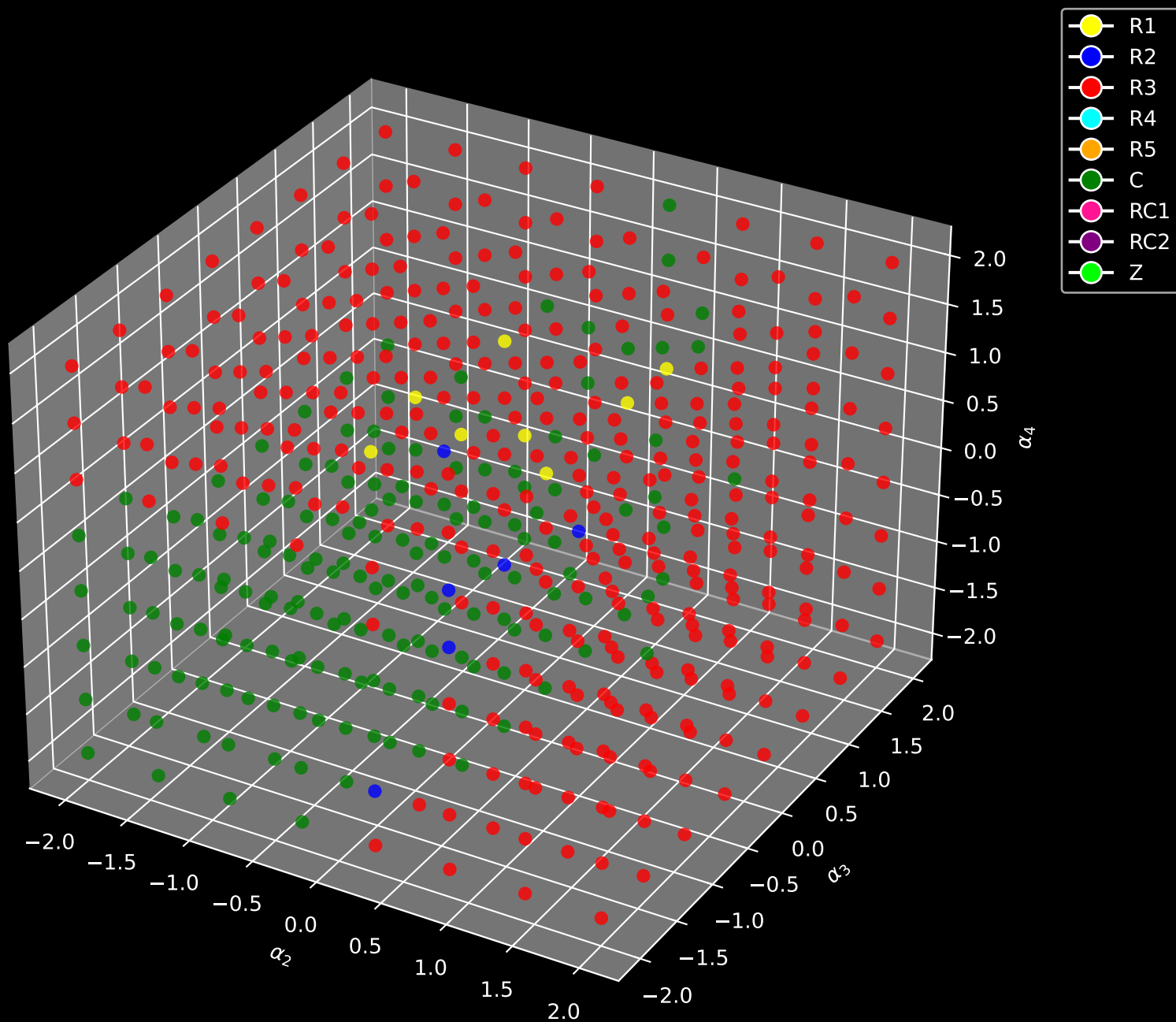
Eigenvalue Categorization (Fixed \alpha_1 = -0.20 )
