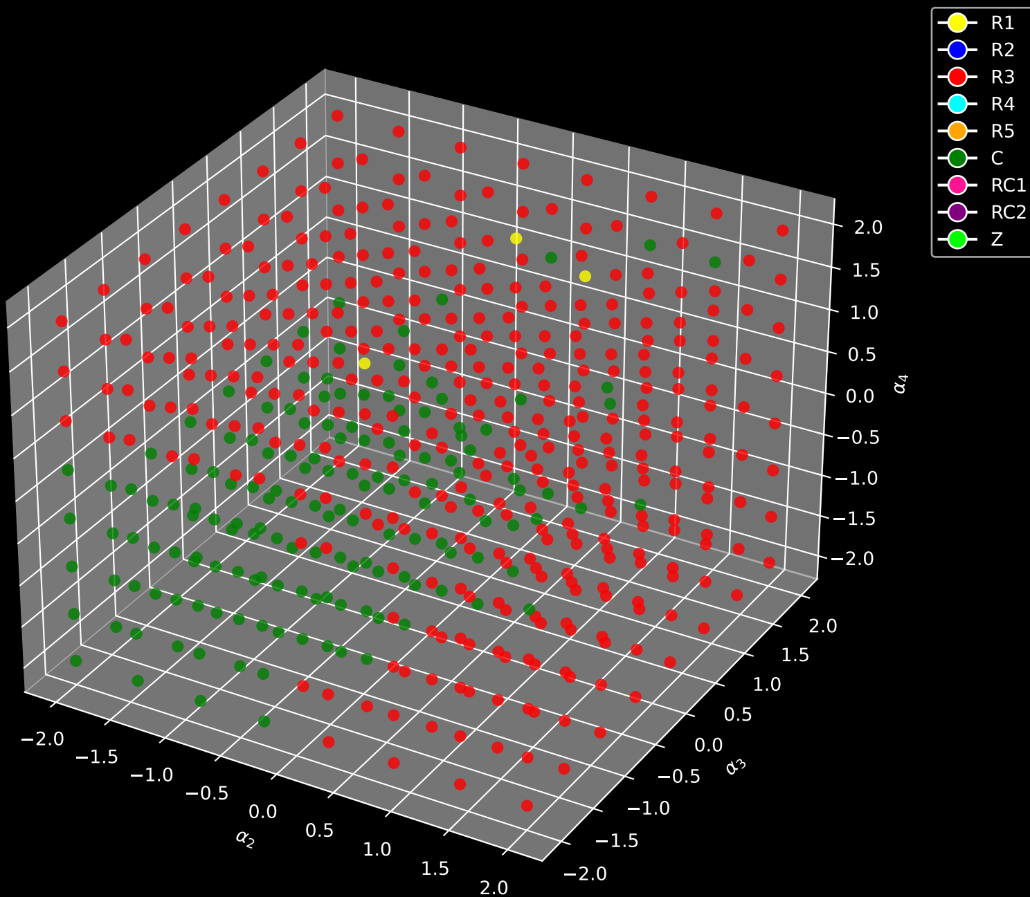
Eigenvalue Categorization (Fixed \alpha_1 = -0.80 )
