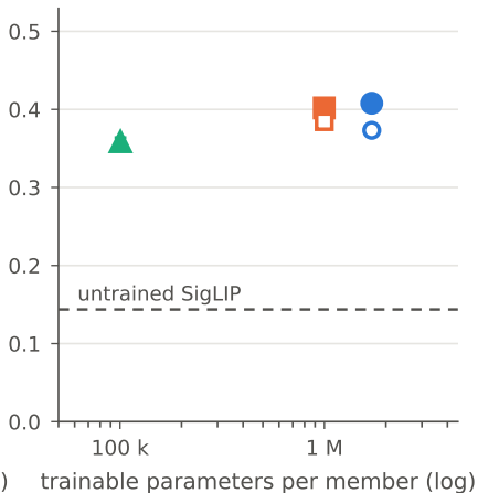
Recall@50
