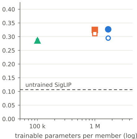
Recall@30
