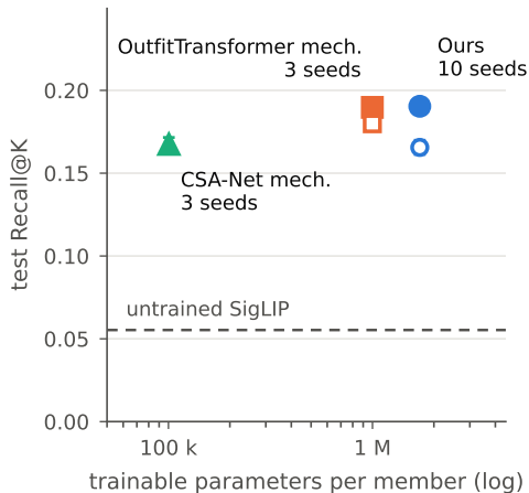
Recall@10
