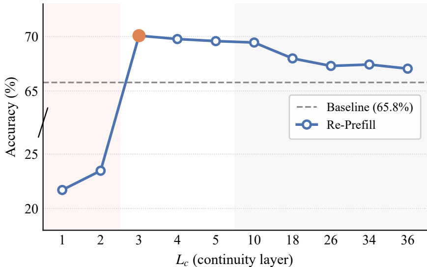
Effect of Continuity Layer L_c on ScreenSpot-Pro
