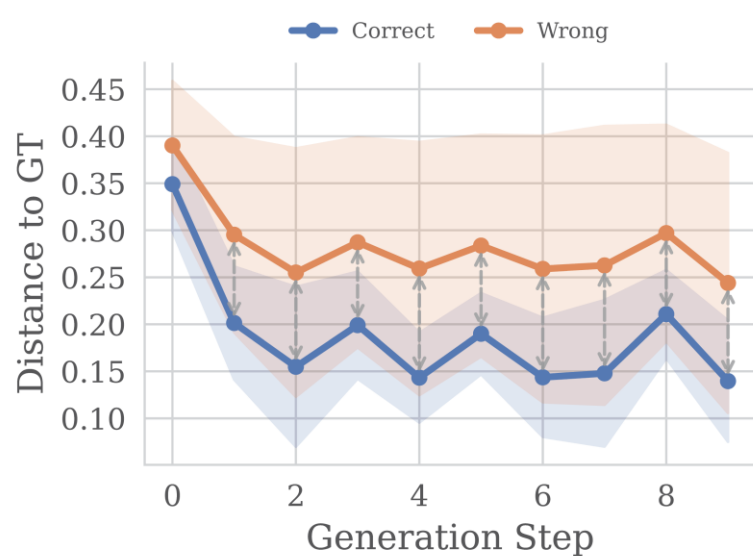
Qwen3-VL-8B-Instruct
