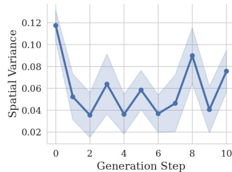
MMBench-GUI
