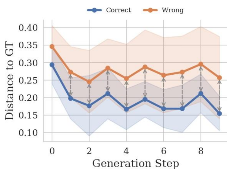
GUI-Owl-1.5-8B-Instruct
