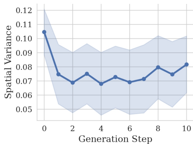
GUI-Owl-1.5-8B-Instruct
