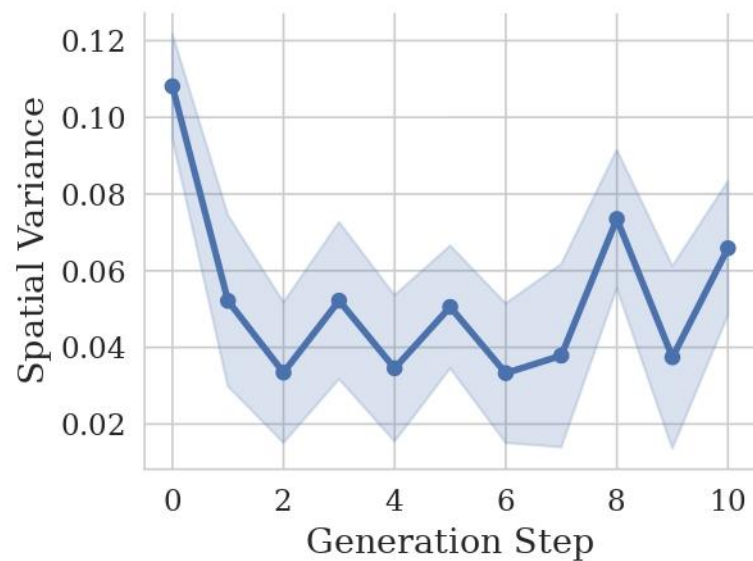
ScreenSpot-Pro
