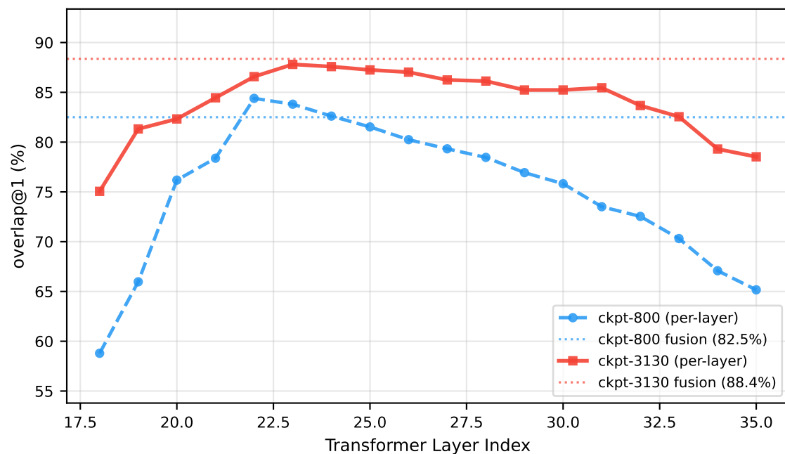
UI-Venus-1.5-8B
