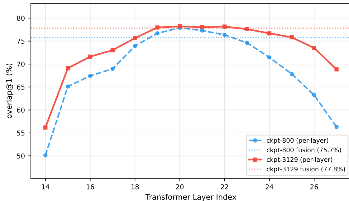
GUI-Owl-1.5-8B
