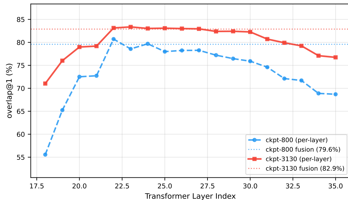
GUI-Owl-1.5-8B
