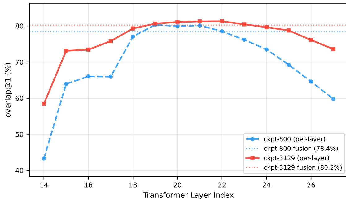
UI-Venus-1.5-8B
