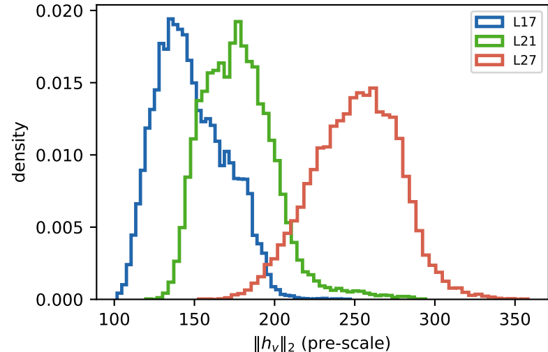
(c) Norm distribution (early/mid/late)
