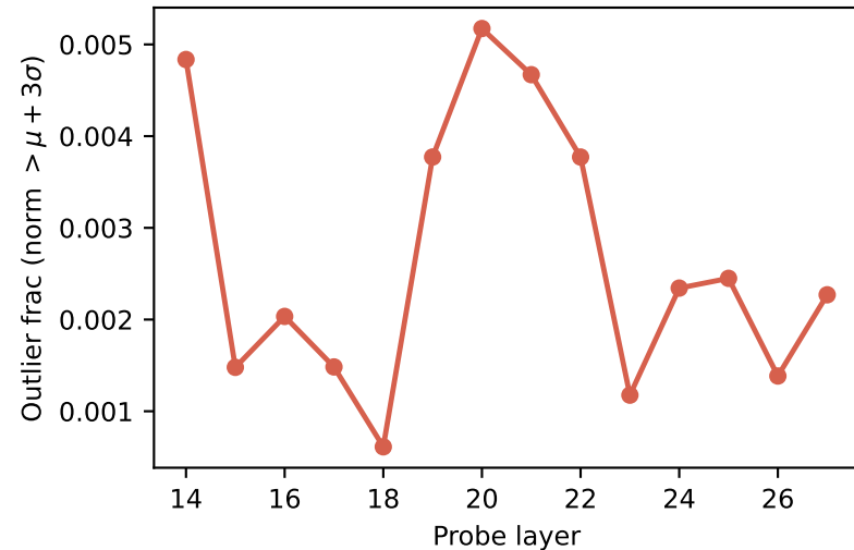
(a) High-norm sink fraction vs depth
