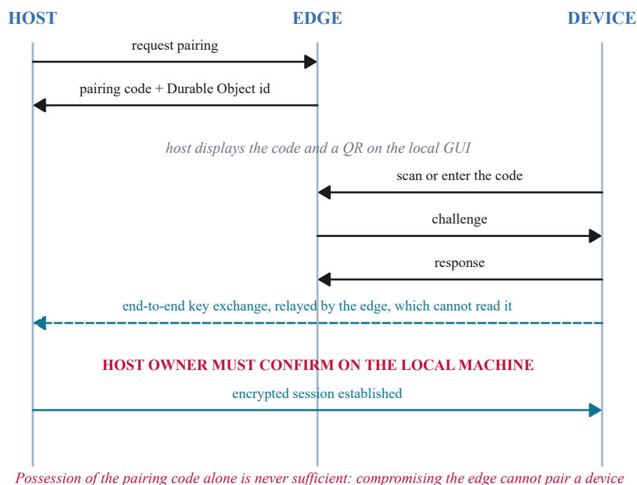
Figure 6.14: The pairing handshake. Host-side confirmation is deliberate, so that possession of the pairing code alone is never sufficient to pair a device.
