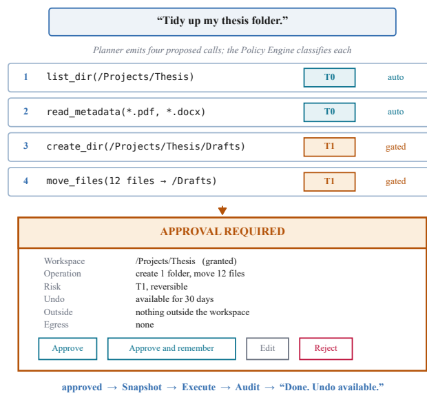
Figure 6.8: A worked classification and approval for a folder tidy. Read operations execute automatically while the reversible operations are gated, and the preview states that nothing leaves the machine and nothing is deleted.
