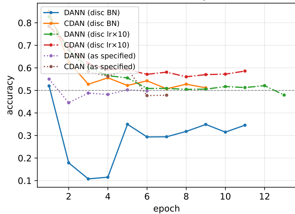
DANN / CDAN discriminator accuracy (dashed = chance)
