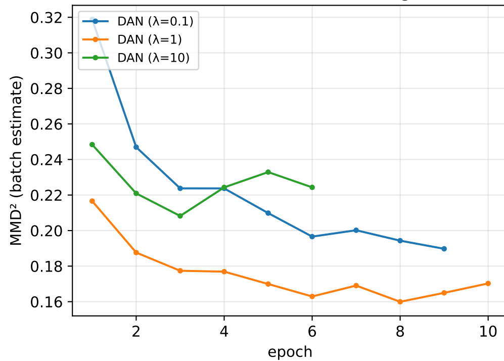
DAN: MK-MMD 2 between source and target features
