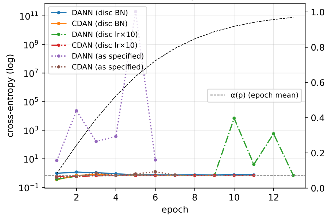
DANN / CDAN domain loss, log scale (dashed = \ln 2 )
