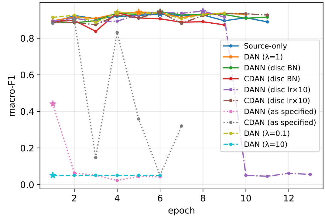
mean source-validation macro-F1 (★ = selected)
