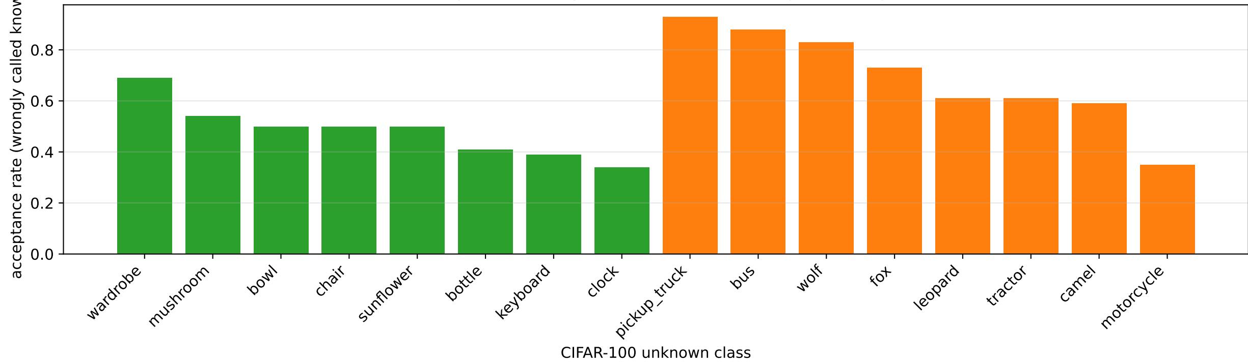
Vanilla + MLS: per-class acceptance of unknowns (orange = near, green = far)
