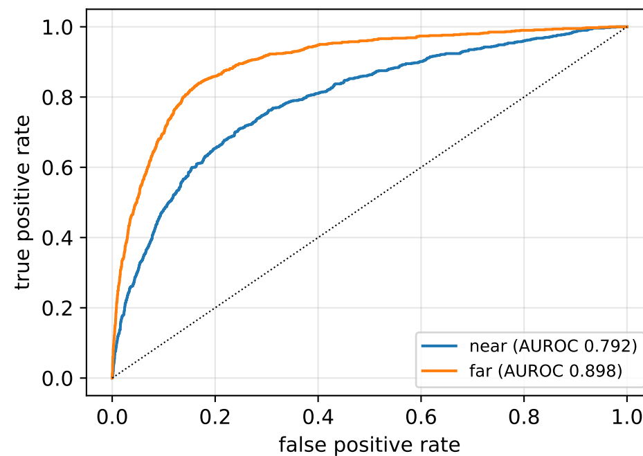
MLS: ROC
