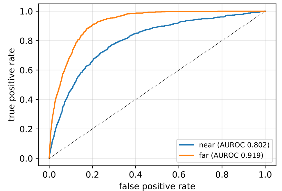
Mahalanobis: ROC
