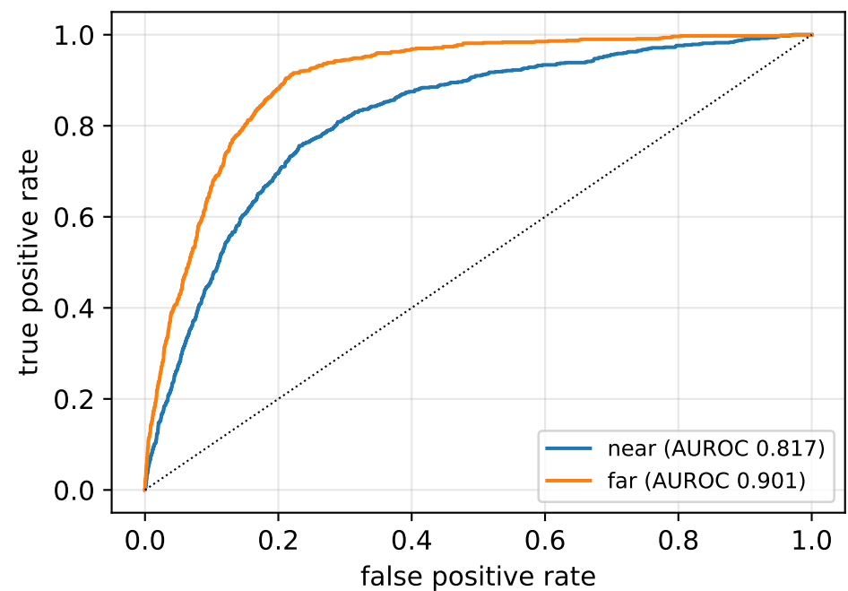
MSP: ROC
