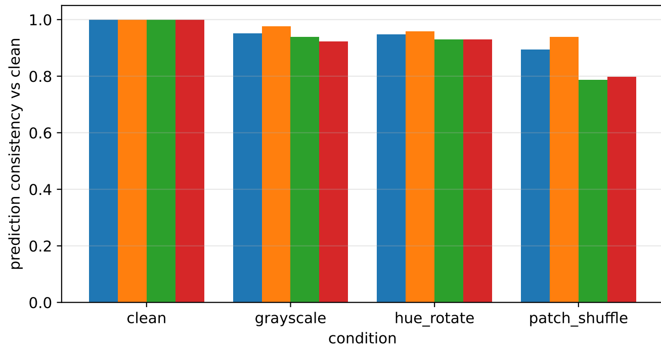
Clean vs colour vs patch-shuffle interventions (500 STL-10 test images)
