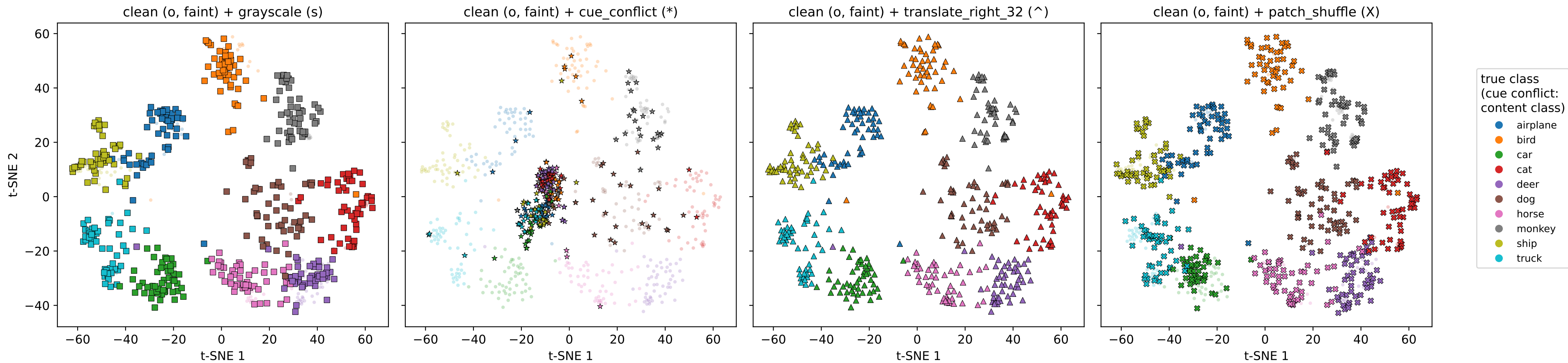
vit_b16: one t-SNE on clean + 4 transformed conditions (perplexity 30, 1000 iters, cosine, seed 6304)
